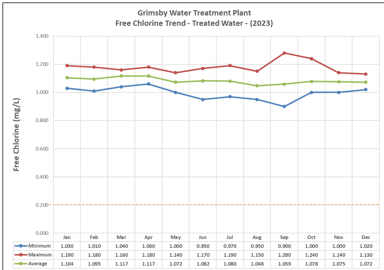
Figure 6-4 Grimsby WTP Treated Water Discharge - Chlorine Residual, 2023
