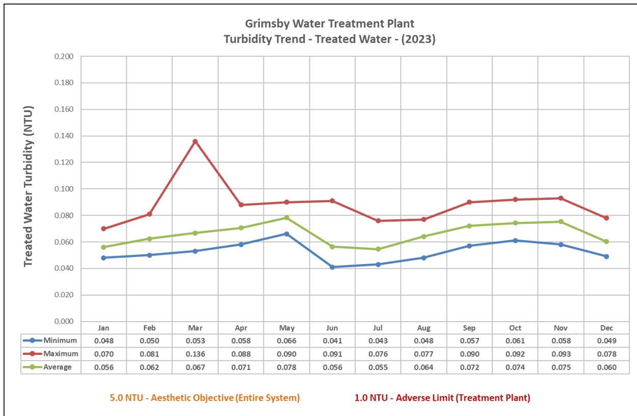
Figure 6-3 Grimsby WTP Treated Water Discharge - Turbidity, 2023
